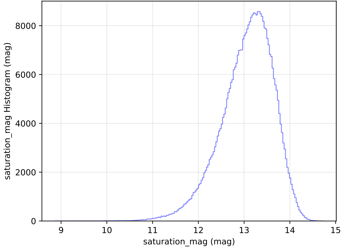
too_elab_r32_d3_ugrizy_v3.4_10yrs WFD y band: saturation_mag Histogram
