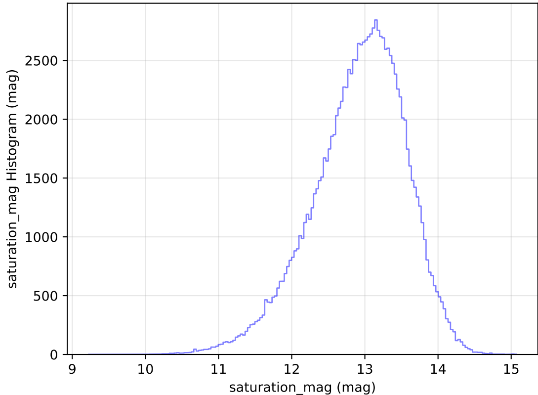
too_elab_r32_d3_ugrizy_v3.4_10yrs WFD u band: saturation_mag Histogram
