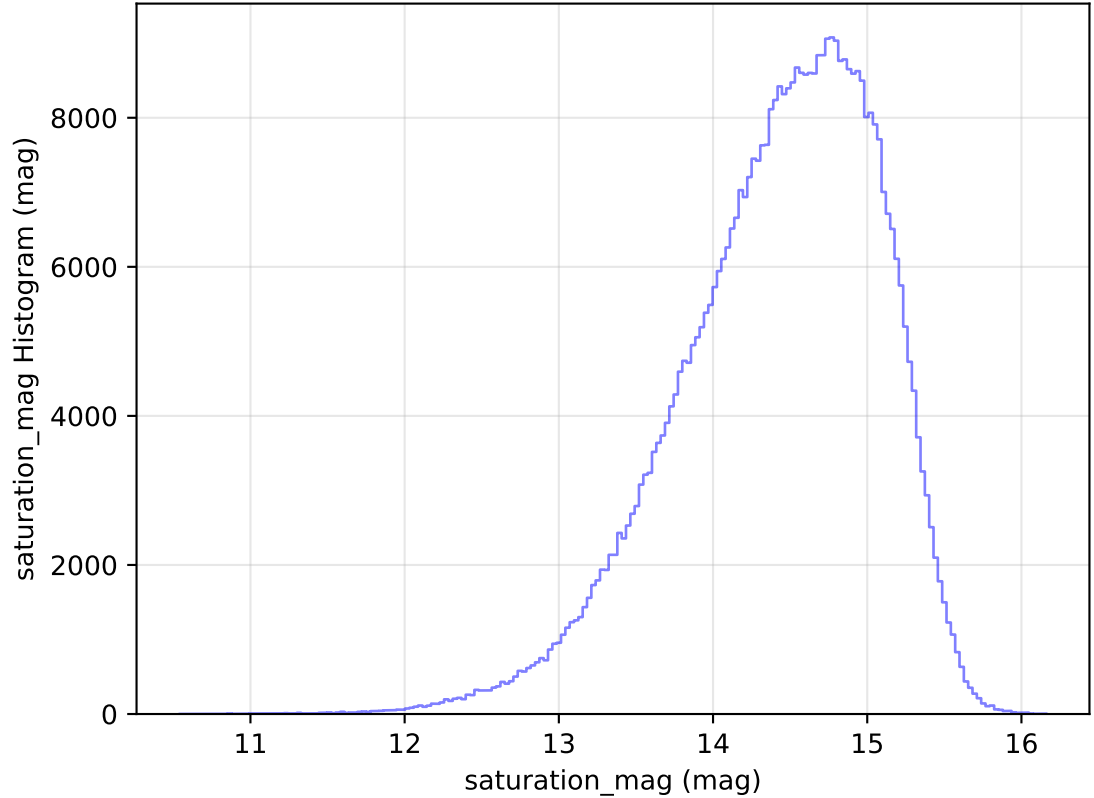
too_elab_r32_d3_ugrizy_v3.4_10yrs WFD i band: saturation_mag Histogram
