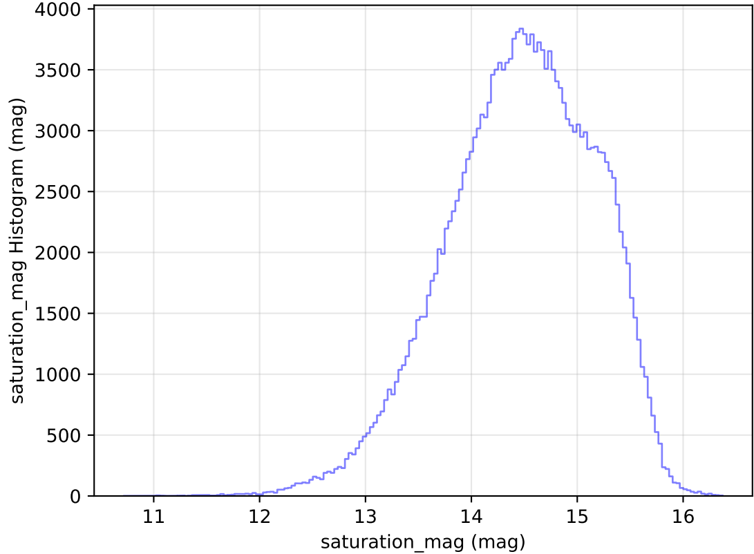
too_elab_r32_d3_ugrizy_v3.4_10yrs WFD g band: saturation_mag Histogram
