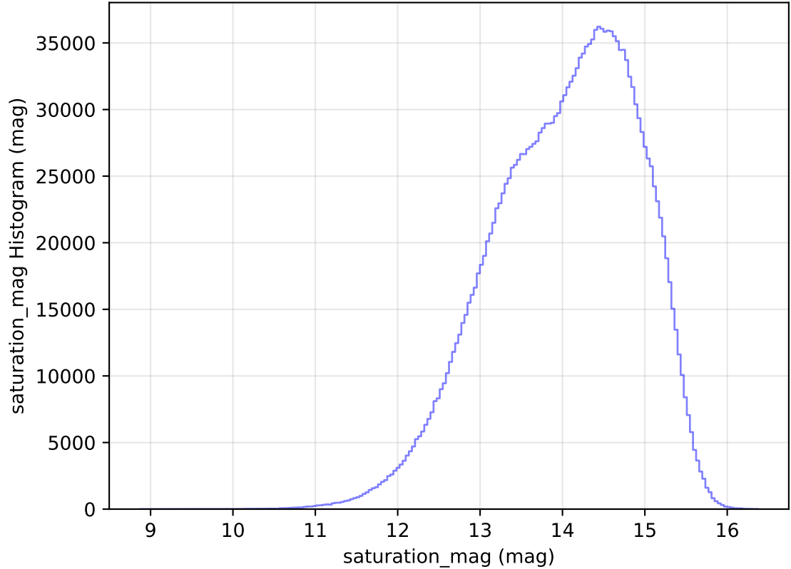
too_elab_r32_d3_ugrizy_v3.4_10yrs WFD all bands: saturation_mag Histogram
