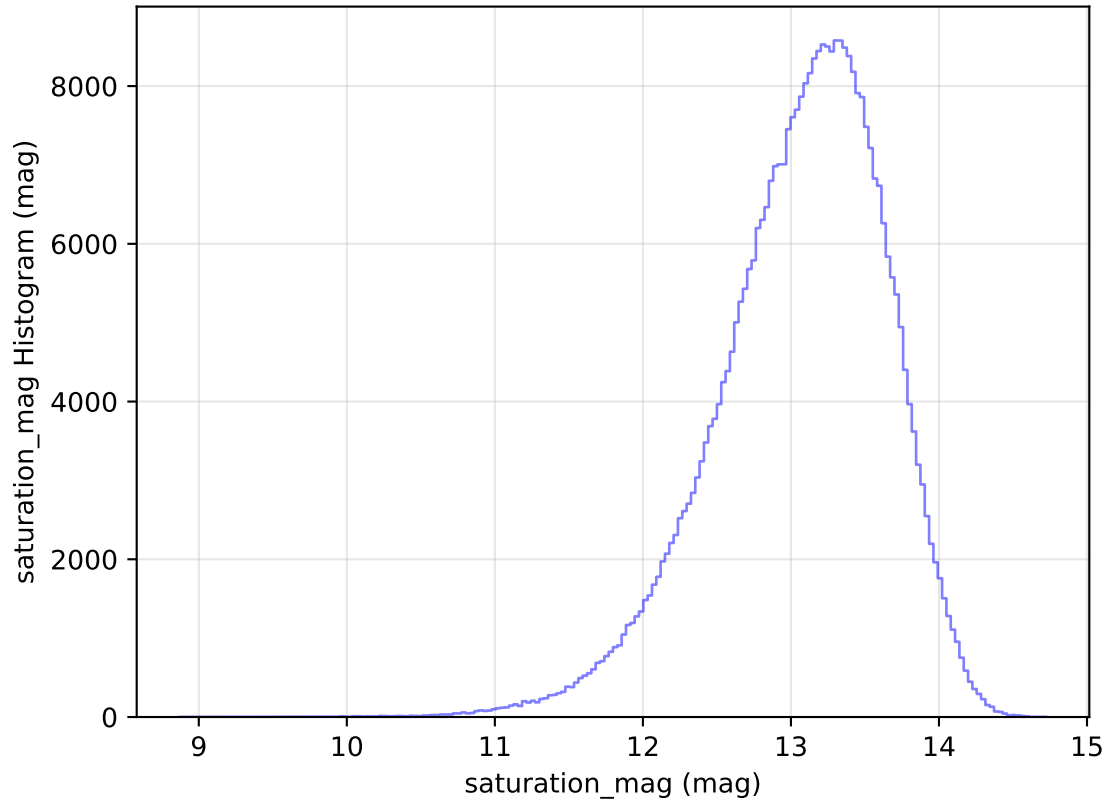
too_elab_r32_d3_ugrizy_v3.4_10yrs All sky y band: saturation_mag Histogram
