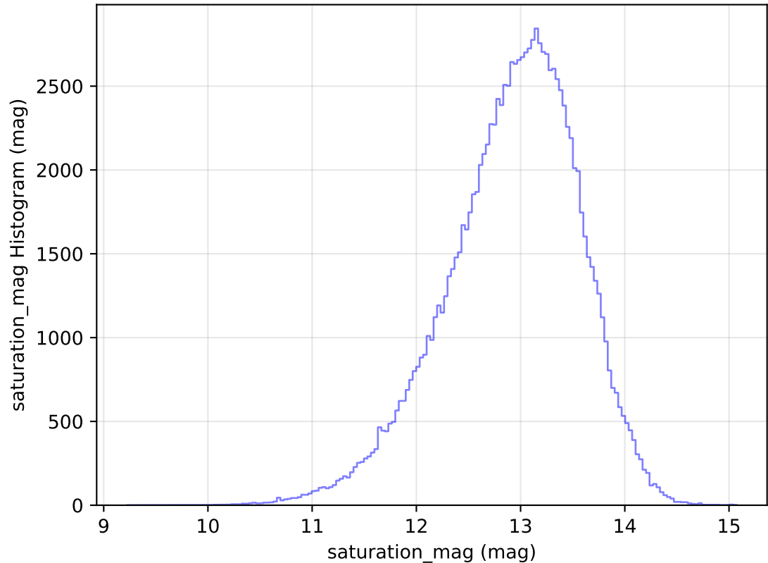
too_elab_r32_d3_ugrizy_v3.4_10yrs All sky u band: saturation_mag Histogram
