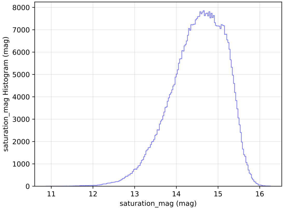
too_elab_r32_d3_ugrizy_v3.4_10yrs All sky r band: saturation_mag Histogram
