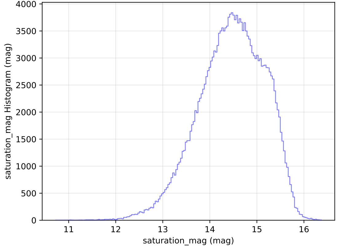
too_elab_r32_d3_ugrizy_v3.4_10yrs All sky g band: saturation_mag Histogram
