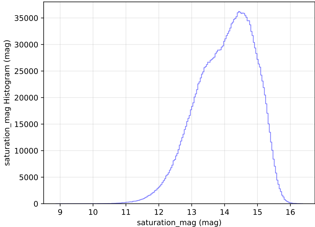
too_elab_r32_d3_ugrizy_v3.4_10yrs All sky all bands: saturation_mag Histogram
