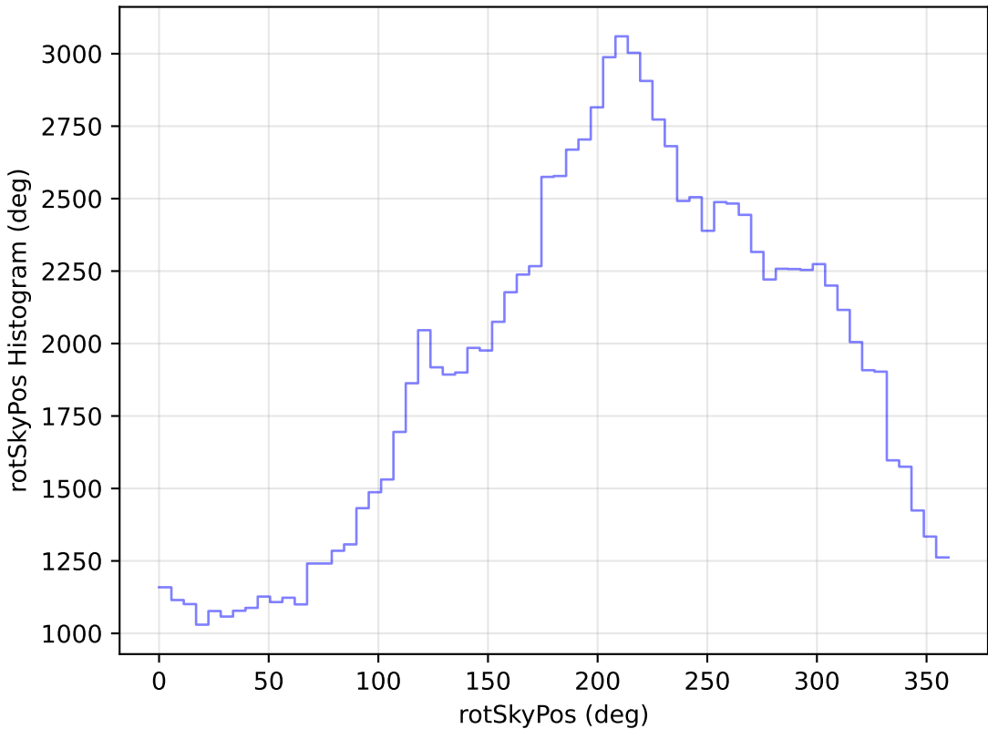
too_elab_r32_d3_ugrizy_v3.4_10yrs WFD u band: rotSkyPos Histogram
