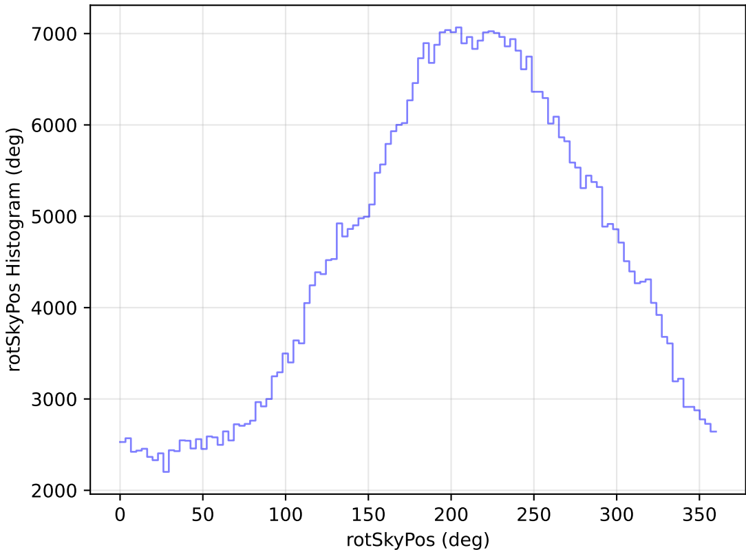
too_elab_r32_d3_ugrizy_v3.4_10yrs WFD i band: rotSkyPos Histogram
