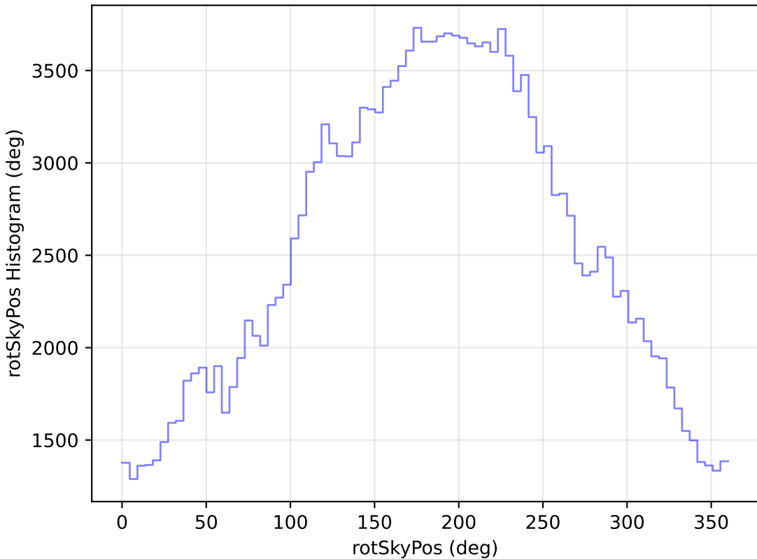
too_elab_r32_d3_ugrizy_v3.4_10yrs WFD g band: rotSkyPos Histogram
