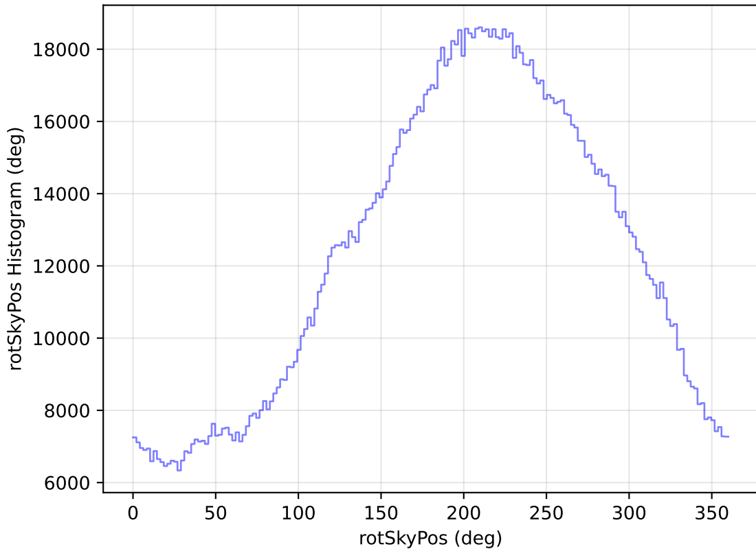
too_elab_r32_d3_ugrizy_v3.4_10yrs WFD all bands: rotSkyPos Histogram
