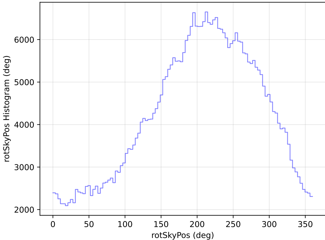
too_elab_r32_d3_ugrizy_v3.4_10yrs All sky z band: rotSkyPos Histogram
