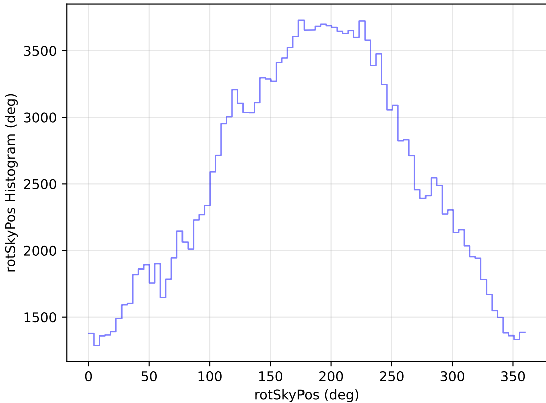
too_elab_r32_d3_ugrizy_v3.4_10yrs All sky g band: rotSkyPos Histogram
