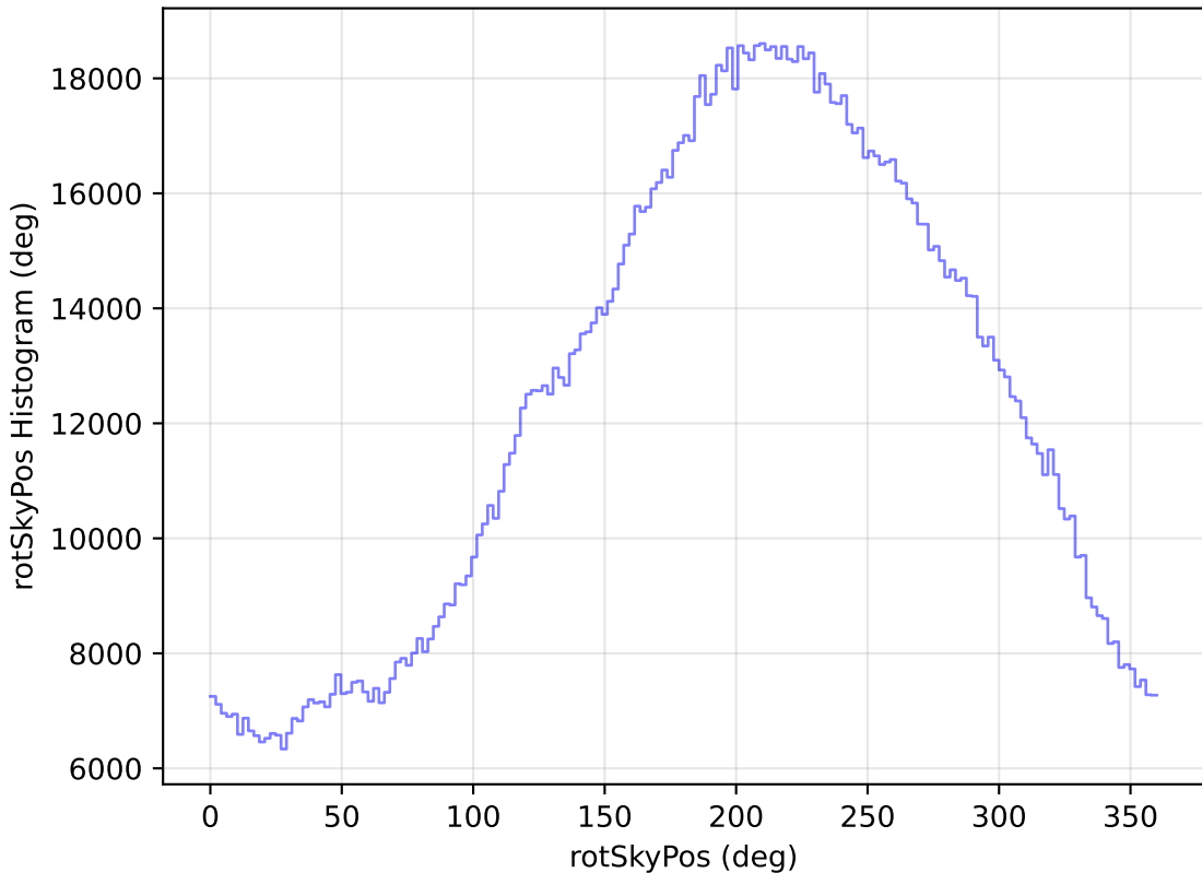
too_elab_r32_d3_ugrizy_v3.4_10yrs All sky all bands: rotSkyPos Histogram
