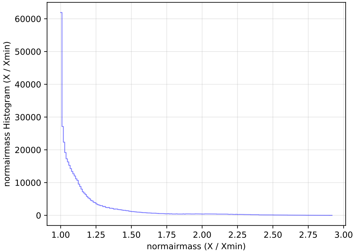
too_elab_r32_d3_ugrizy_v3.4_10yrs WFD z band: normairmass Histogram
