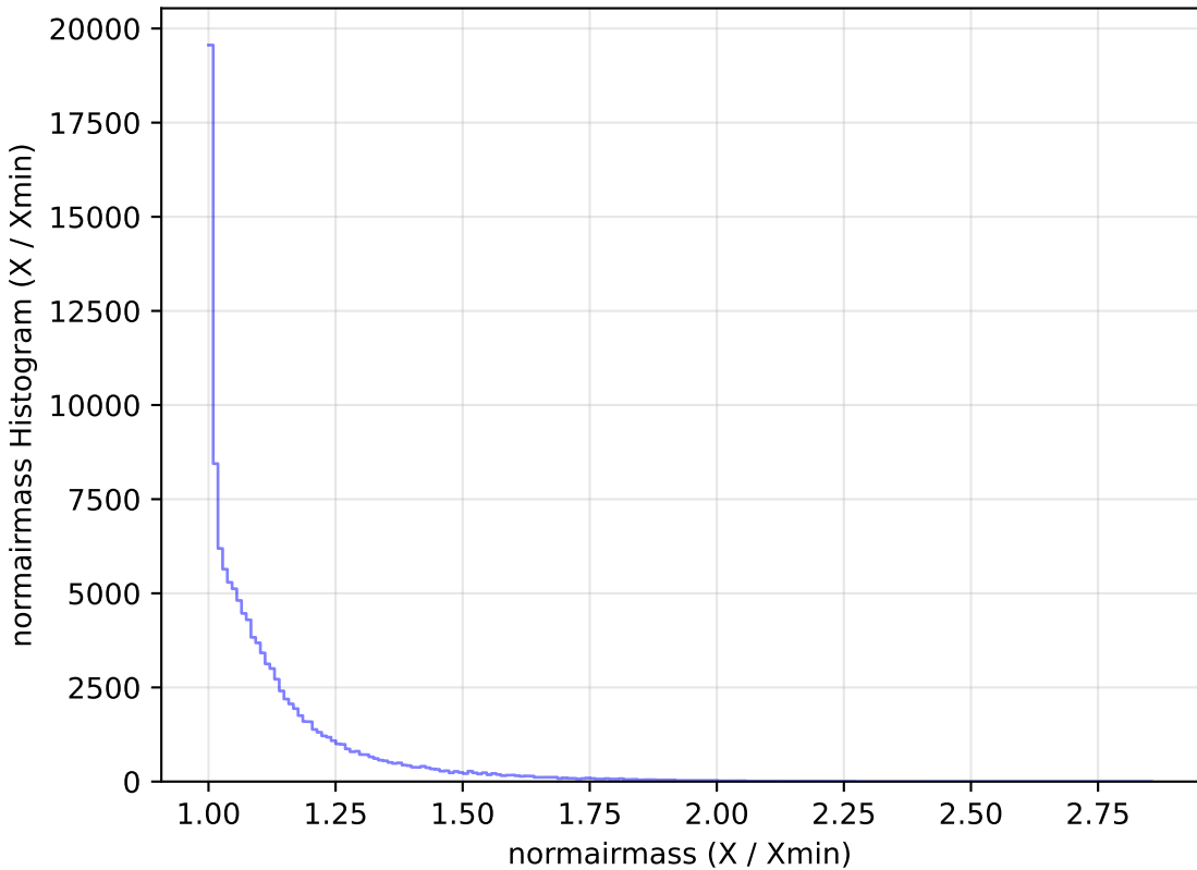
too_elab_r32_d3_ugrizy_v3.4_10yrs WFD u band: normairmass Histogram
