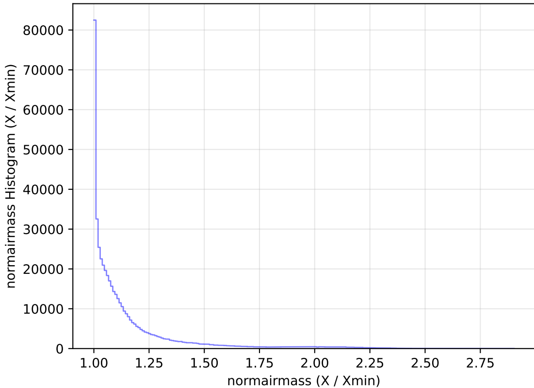
too_elab_r32_d3_ugrizy_v3.4_10yrs WFD r band: normairmass Histogram
