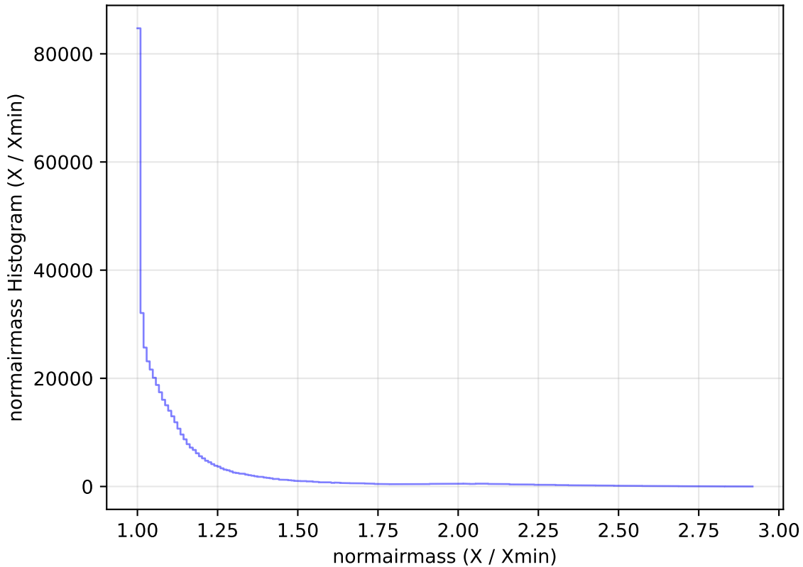
too_elab_r32_d3_ugrizy_v3.4_10yrs WFD i band: normairmass Histogram
