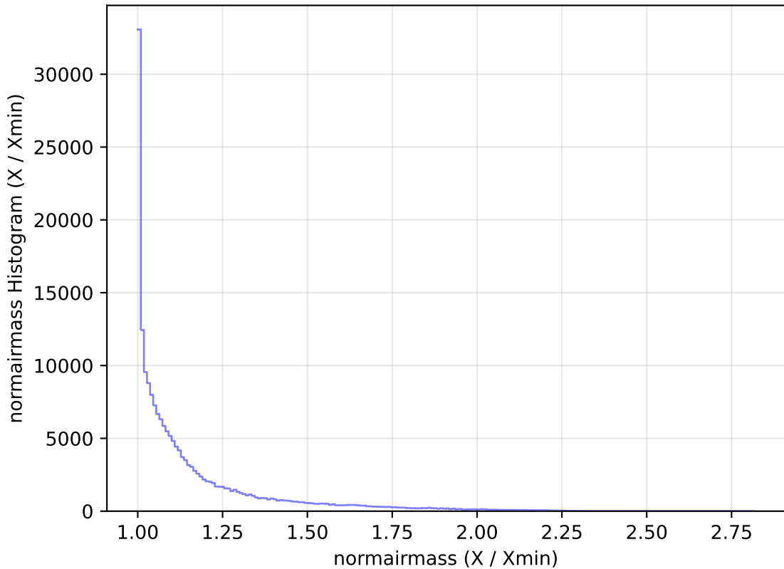
too_elab_r32_d3_ugrizy_v3.4_10yrs WFD g band: normairmass Histogram
