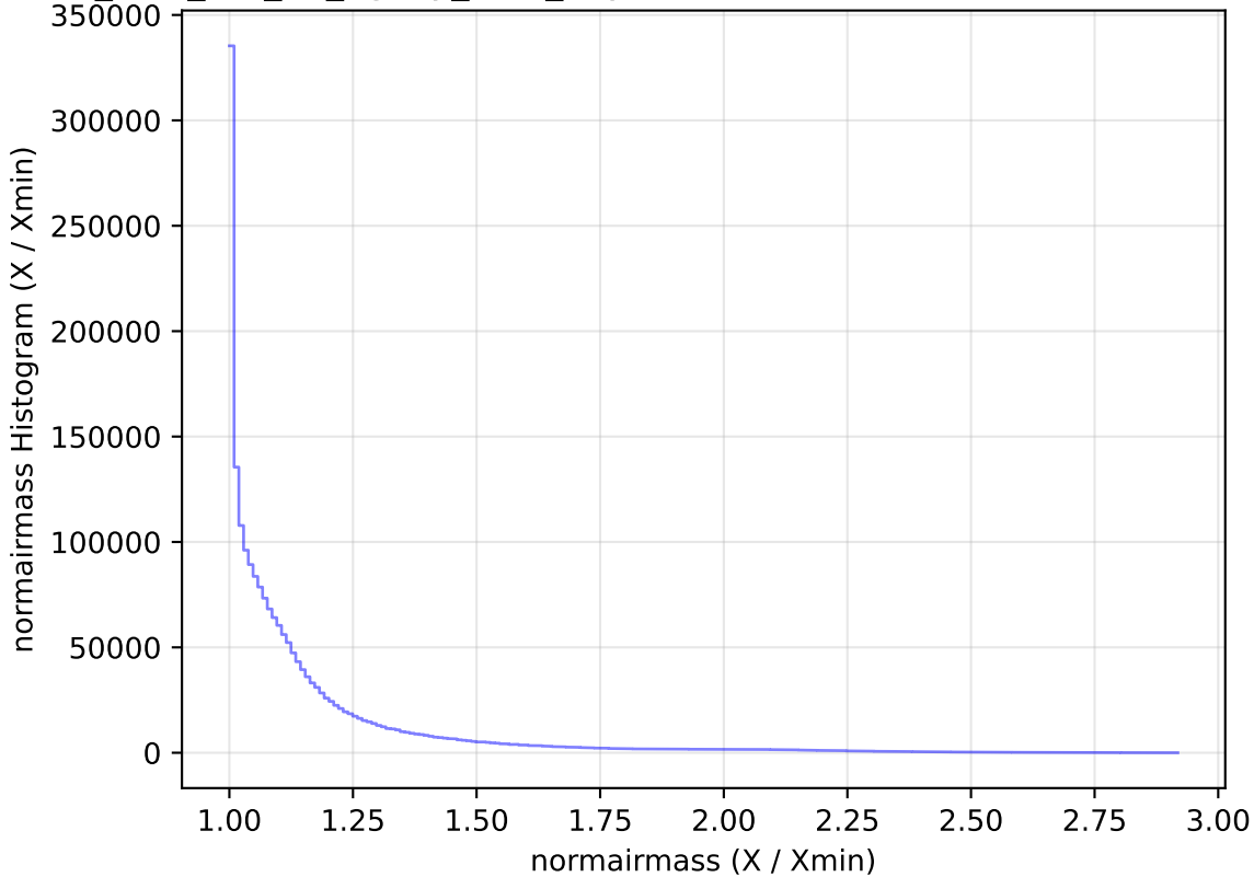
too_elab_r32_d3_ugrizy_v3.4_10yrs WFD all bands: normairmass Histogram
