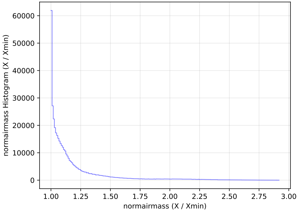
too_elab_r32_d3_ugrizy_v3.4_10yrs All sky z band: normairmass Histogram
