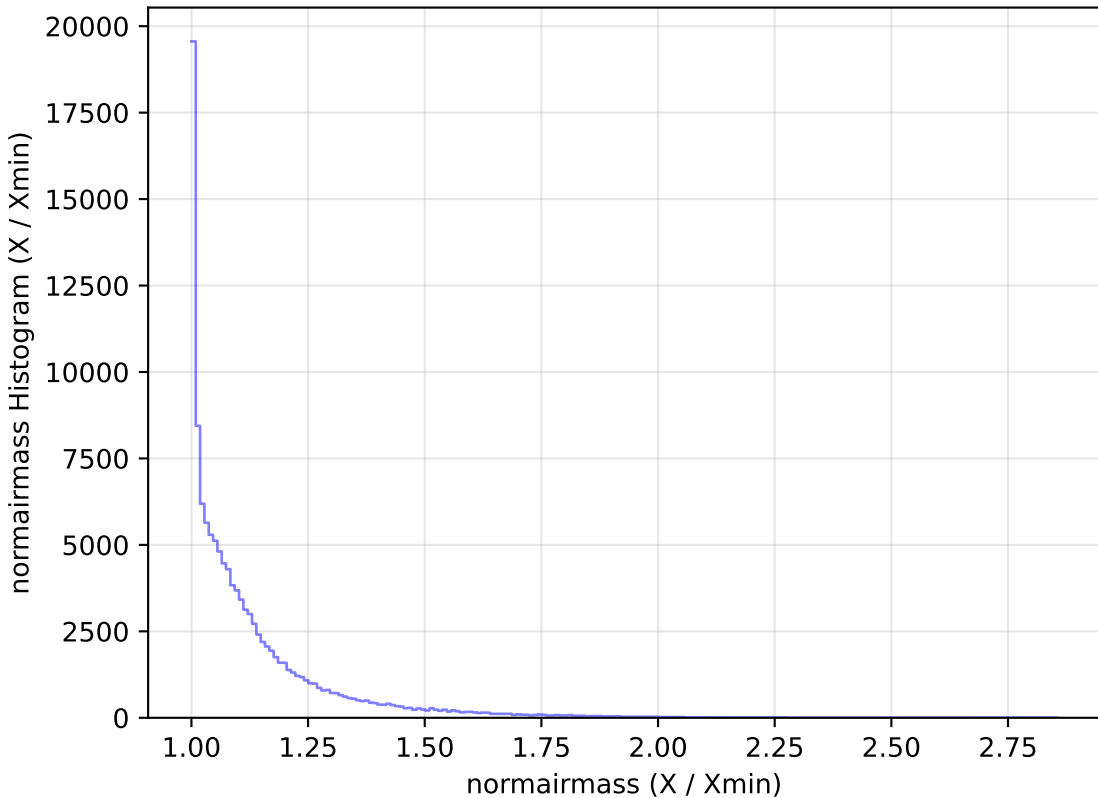
too_elab_r32_d3_ugrizy_v3.4_10yrs All sky u band: normairmass Histogram
