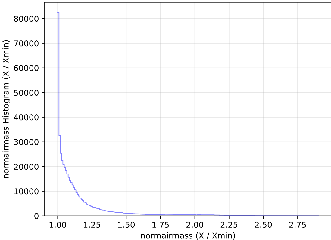
too_elab_r32_d3_ugrizy_v3.4_10yrs All sky r band: normairmass Histogram
