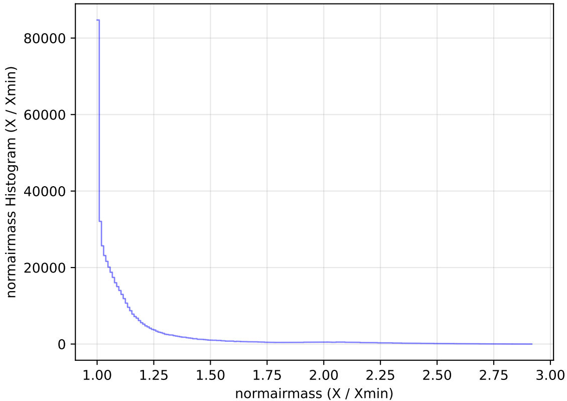
too_elab_r32_d3_ugrizy_v3.4_10yrs All sky i band: normairmass Histogram
