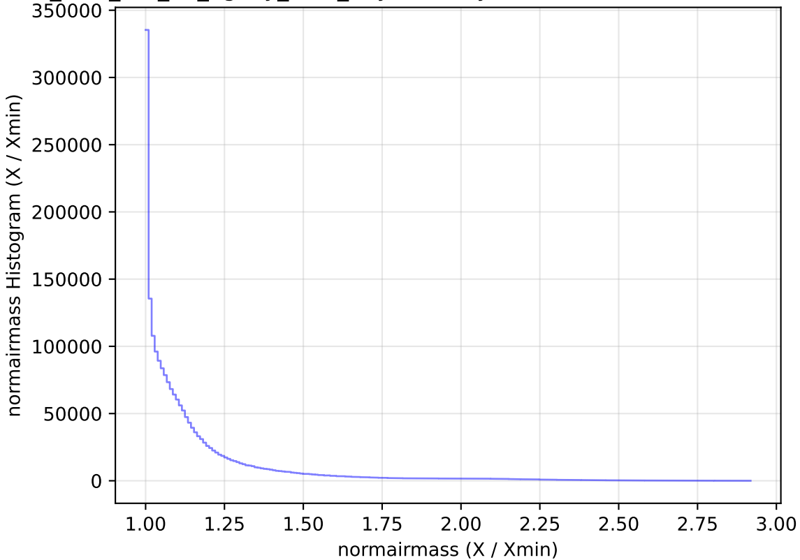
too_elab_r32_d3_ugrizy_v3.4_10yrs All sky all bands: normairmass Histogram
