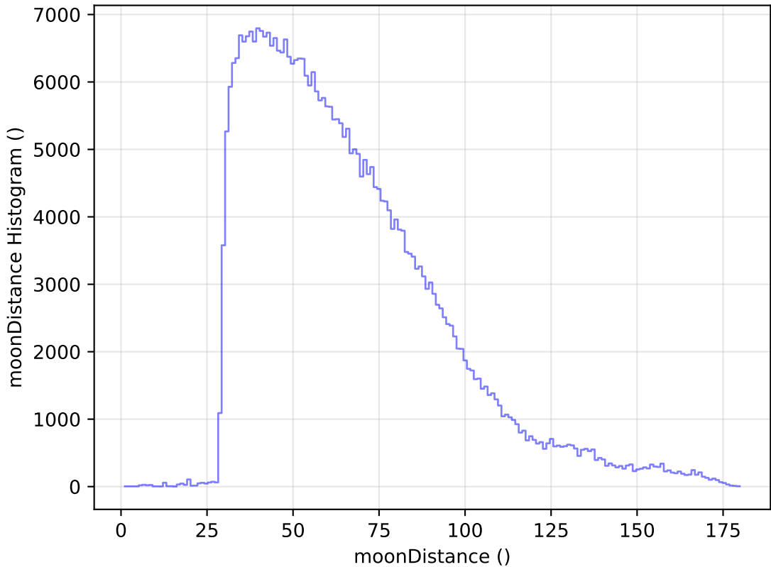
too_elab_r32_d3_ugrizy_v3.4_10yrs WFD y band: moonDistance Histogram
