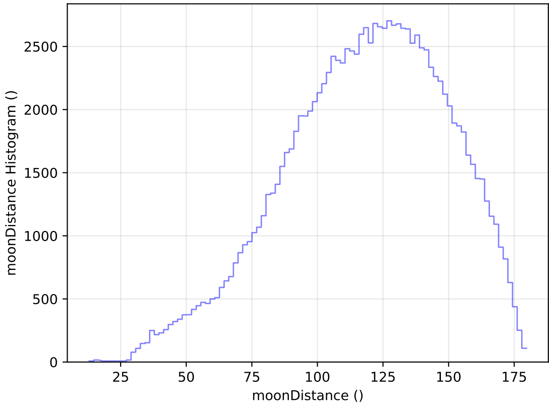
too_elab_r32_d3_ugrizy_v3.4_10yrs WFD u band: moonDistance Histogram
