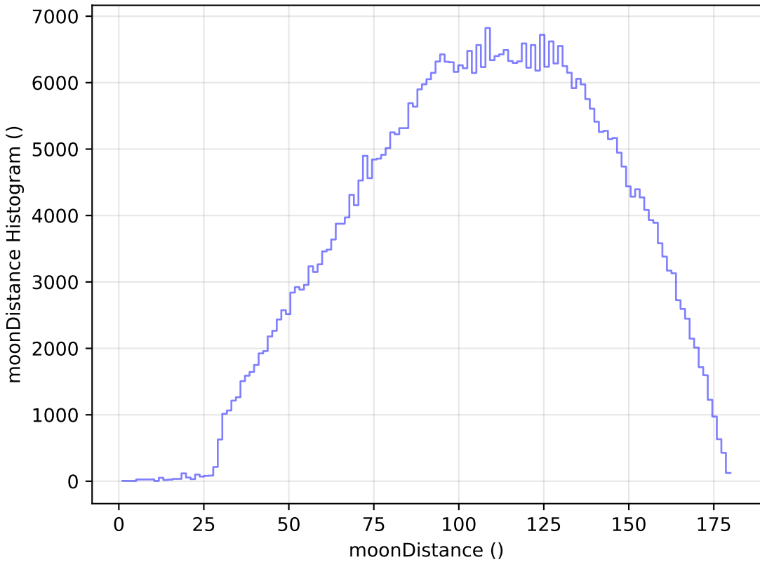
too_elab_r32_d3_ugrizy_v3.4_10yrs WFD r band: moonDistance Histogram
