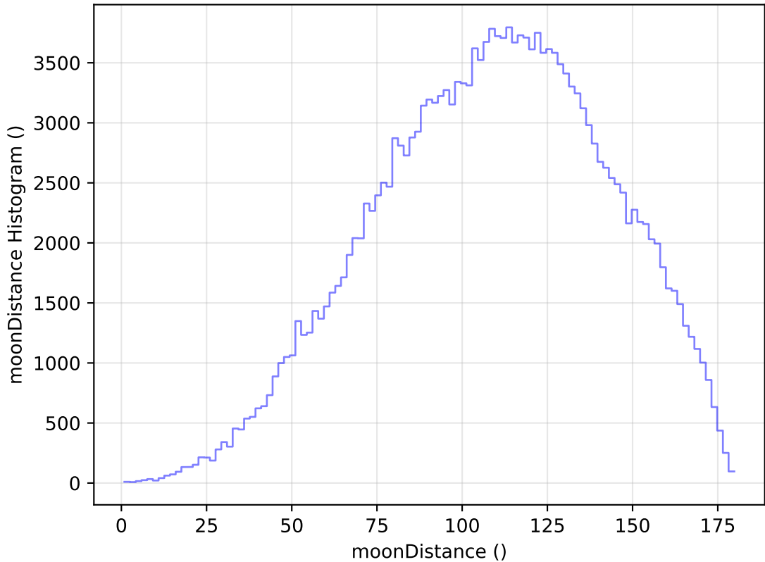
too_elab_r32_d3_ugrizy_v3.4_10yrs WFD g band: moonDistance Histogram
