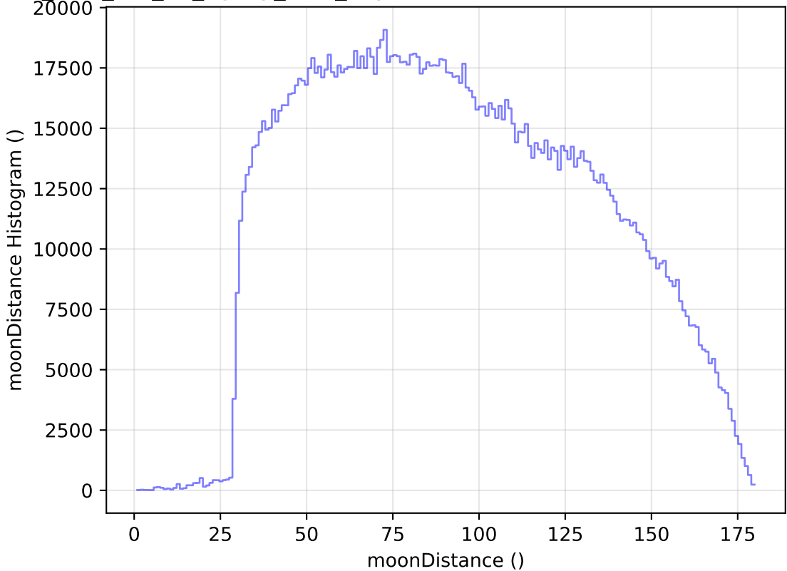
too_elab_r32_d3_ugrizy_v3.4_10yrs WFD all bands: moonDistance Histogram
