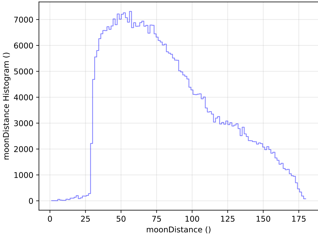
too_elab_r32_d3_ugrizy_v3.4_10yrs All sky z band: moonDistance Histogram
