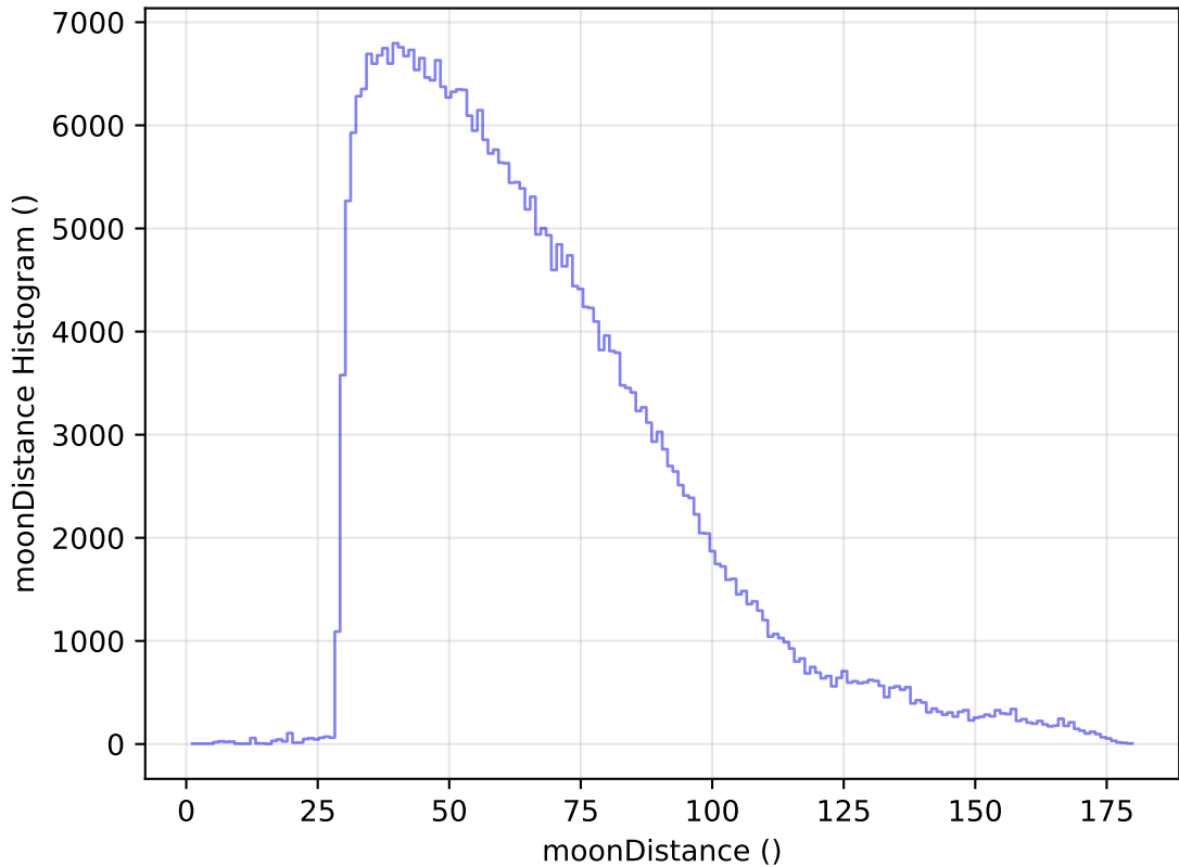
too_elab_r32_d3_ugrizy_v3.4_10yrs All sky y band: moonDistance Histogram
