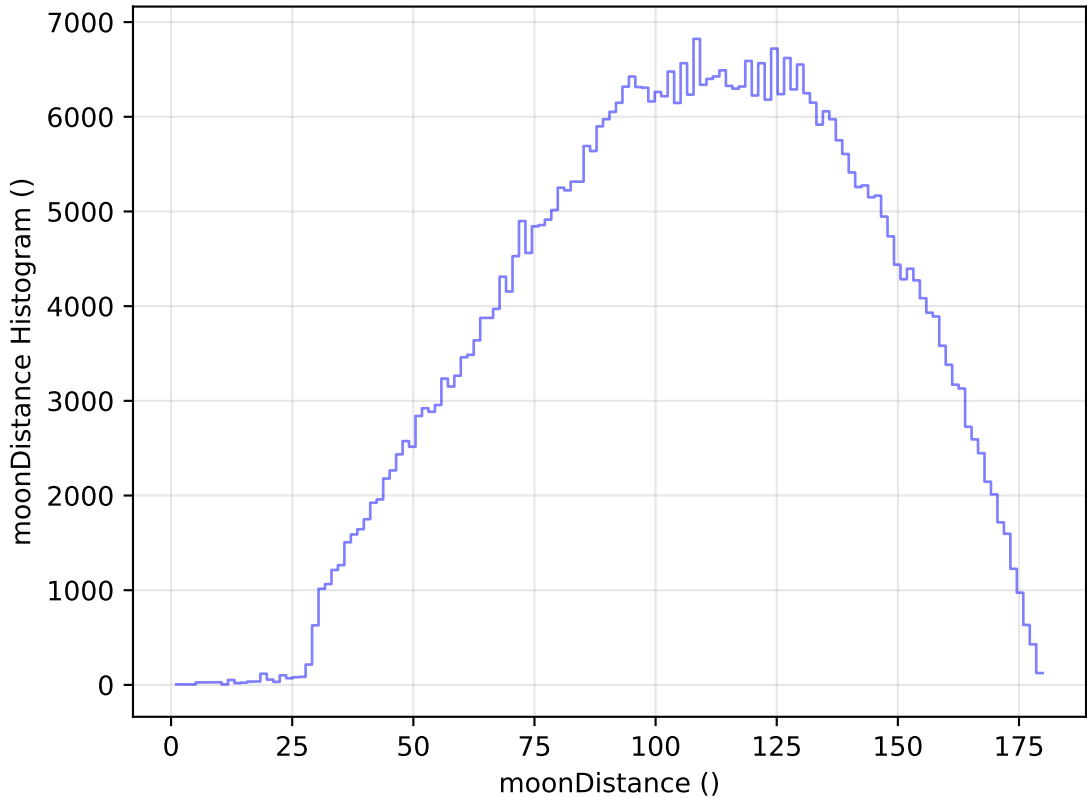
too_elab_r32_d3_ugrizy_v3.4_10yrs All sky r band: moonDistance Histogram
