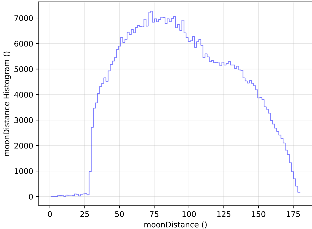
too_elab_r32_d3_ugrizy_v3.4_10yrs All sky i band: moonDistance Histogram
