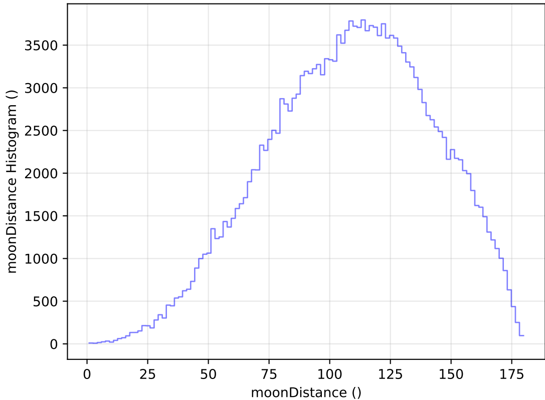
too_elab_r32_d3_ugrizy_v3.4_10yrs All sky g band: moonDistance Histogram
