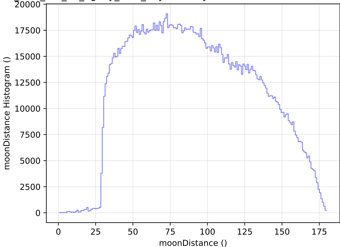
too_elab_r32_d3_ugrizy_v3.4_10yrs All sky all bands: moonDistance Histogram
