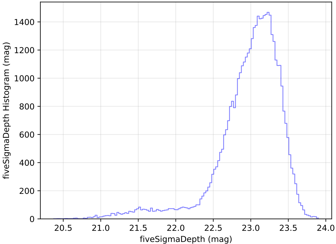
too_elab_r32_d3_ugrizy_v3.4_10yrs Yr 1 z band: fiveSigmaDepth Histogram
