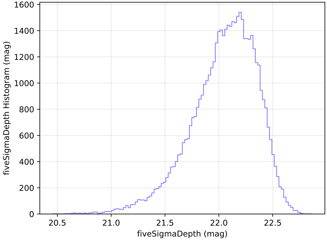
too_elab_r32_d3_ugrizy_v3.4_10yrs Yr 1 y band: fiveSigmaDepth Histogram
