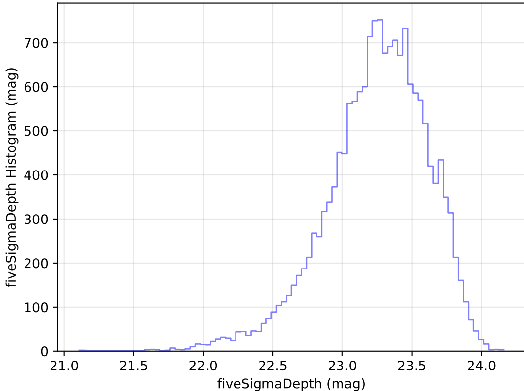
too_elab_r32_d3_ugrizy_v3.4_10yrs Yr 1 u band: fiveSigmaDepth Histogram
