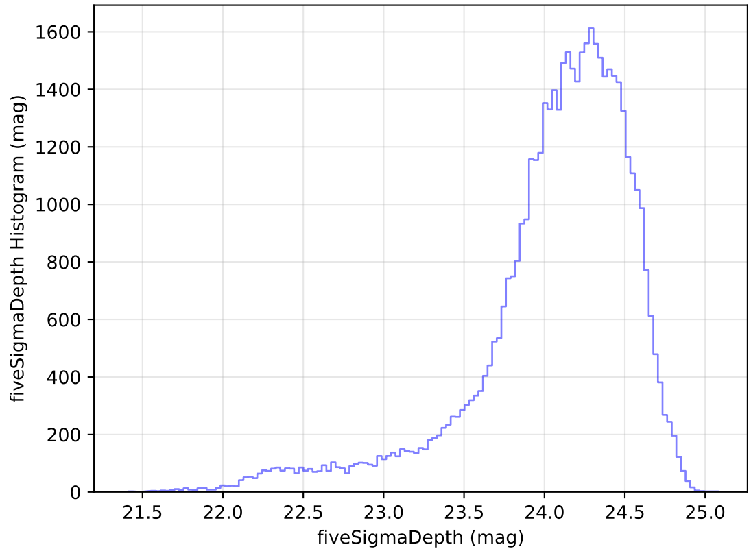
too_elab_r32_d3_ugrizy_v3.4_10yrs Yr 1 r band: fiveSigmaDepth Histogram
