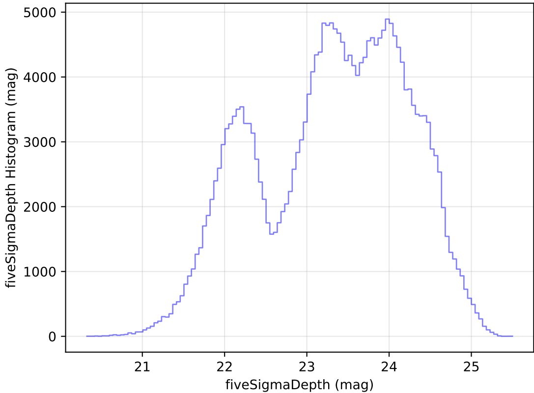
too_elab_r32_d3_ugrizy_v3.4_10yrs Yr 1 all bands: fiveSigmaDepth Histogram
