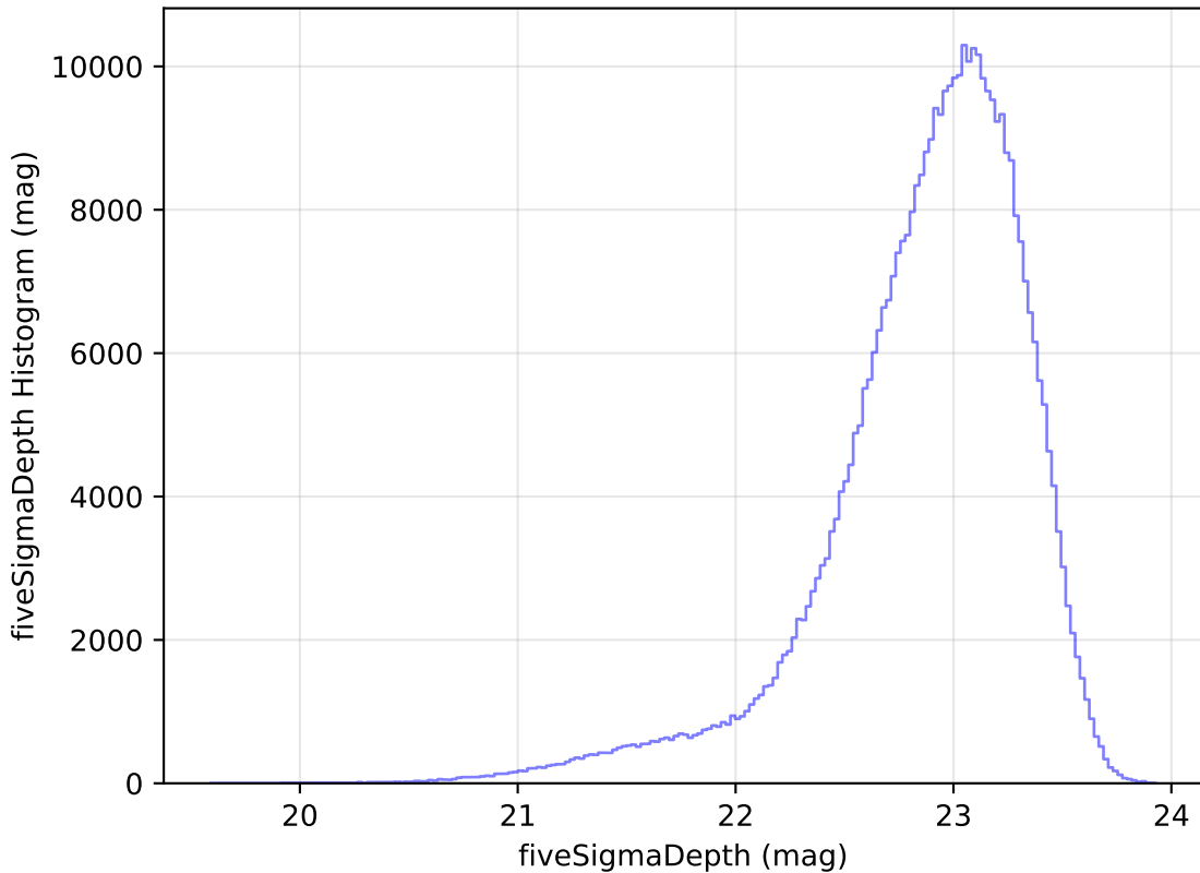
too_elab_r32_d3_ugrizy_v3.4_10yrs WFD z band: fiveSigmaDepth Histogram
