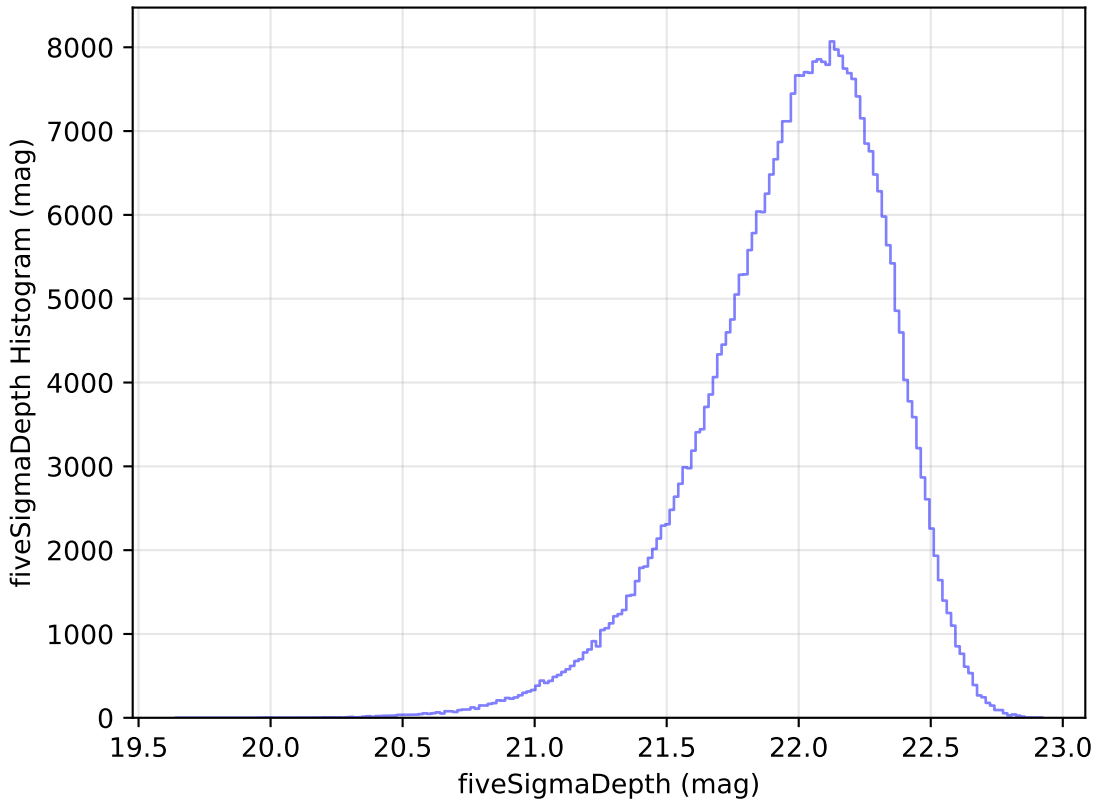
too_elab_r32_d3_ugrizy_v3.4_10yrs WFD y band: fiveSigmaDepth Histogram
