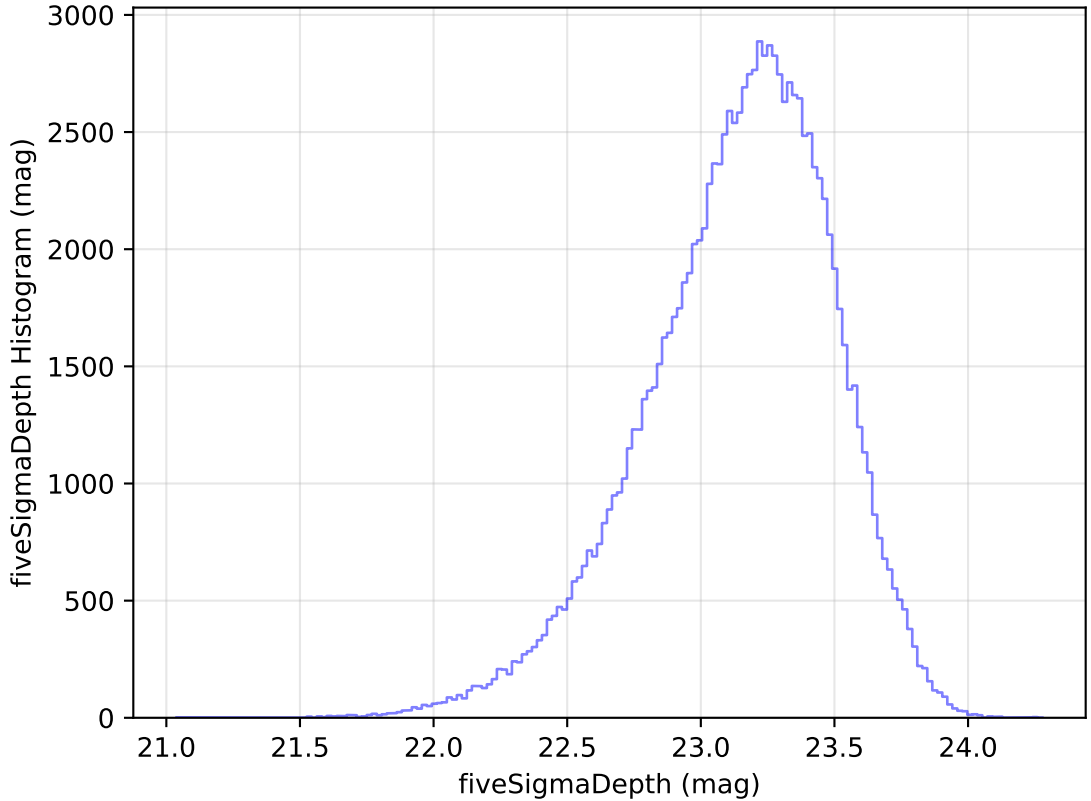
too_elab_r32_d3_ugrizy_v3.4_10yrs WFD u band: fiveSigmaDepth Histogram
