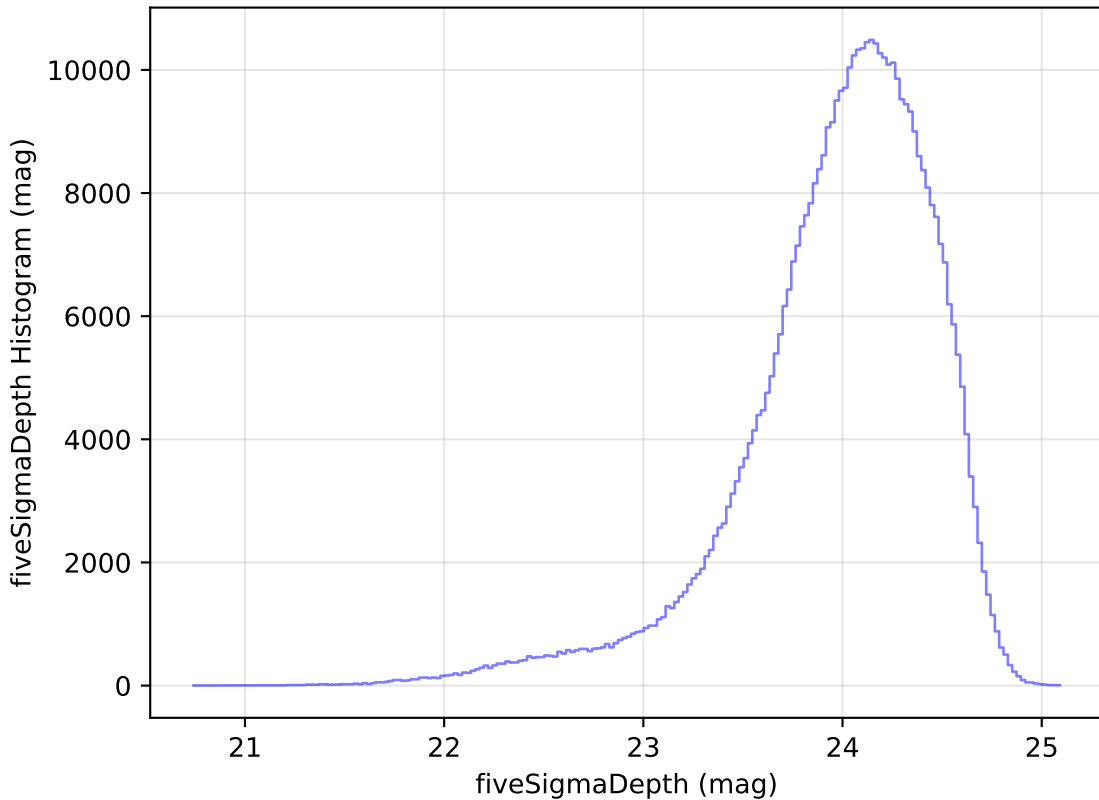
too_elab_r32_d3_ugrizy_v3.4_10yrs WFD r band: fiveSigmaDepth Histogram
