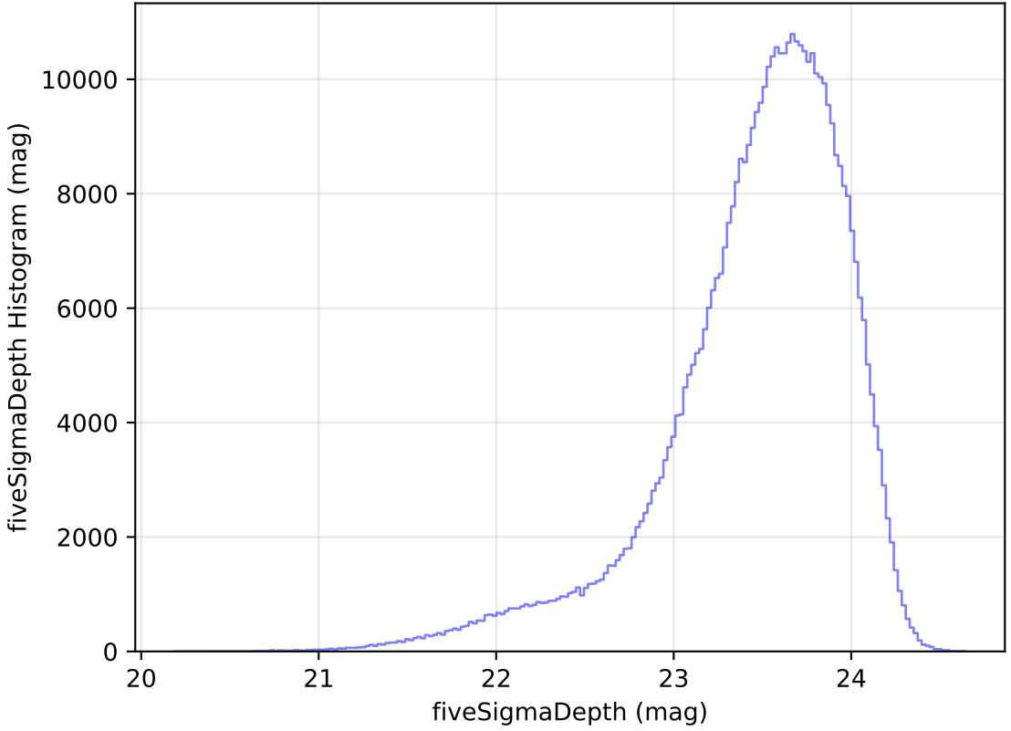
too_elab_r32_d3_ugrizy_v3.4_10yrs WFD i band: fiveSigmaDepth Histogram
