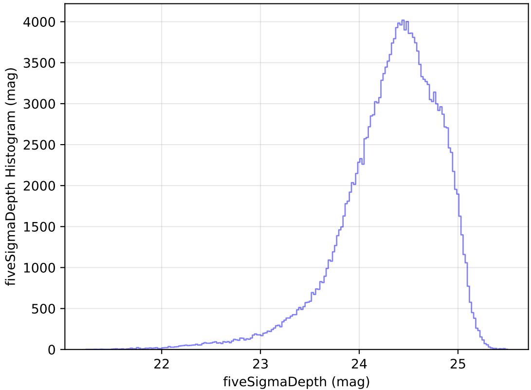
too_elab_r32_d3_ugrizy_v3.4_10yrs WFD g band: fiveSigmaDepth Histogram
